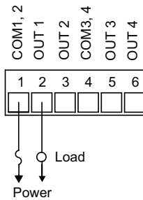
Relay Version
